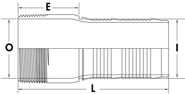
Insta-Lock™ Interlocking Stainless Steel Male NPT Hose Stem
