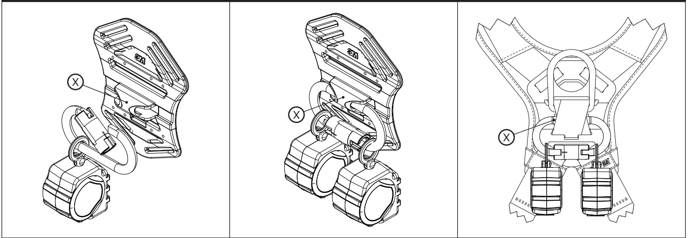
Figure 10C - Interface Loop
