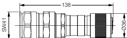
Inlet metal version: V > 2000 cm 3
