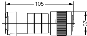
Plug plastic version
