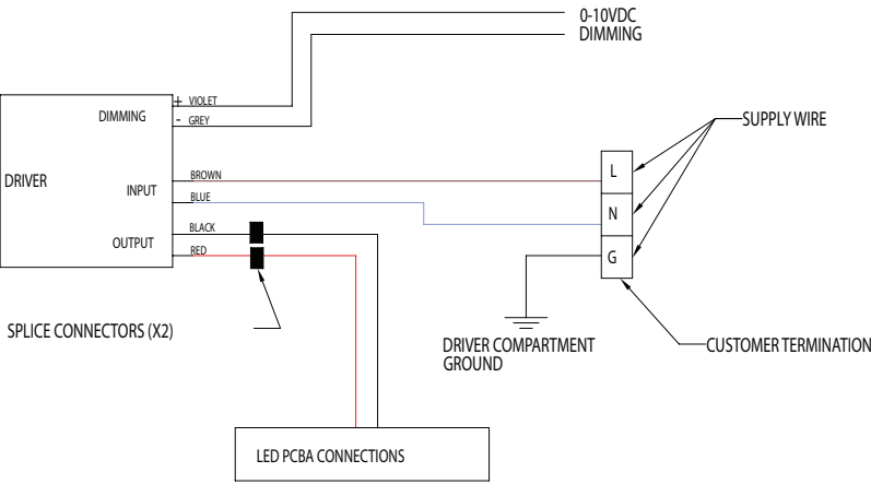
WIRING DIAGRAM 3L/5L/7L/9L DRIVER CONFIGURATION
