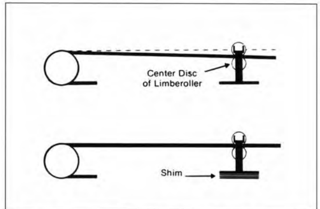
Figure 3 Relationship of Limberoller idler and pulleys
