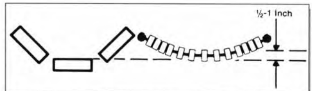
Figure 2 Position of Limberoller idler in relation to steel roll
