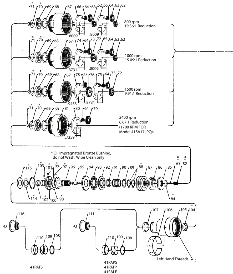
Figure 1. Exploded View - TPA898-4
