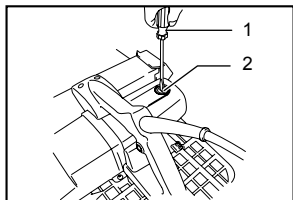
1. Screwdriver 2. Brush holder cap
